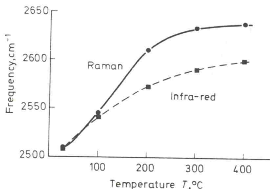
Figure 8. Frequency shift of OD-vibration of HDO in \text{H}_2\text{O} with temperature at constant density of 1.0 \text{ g/cm}^3 .
